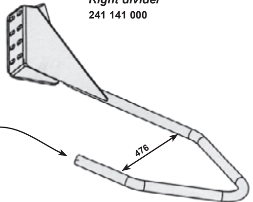
Diviseur droit large Large right divider
